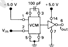
FIGURE 3 — VOLTAGE-CONTROLLED MULTIVIBRATOR
