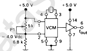
FIGURE 2 — CRYSTAL CONTROLLED MULTIVIBRATOR
